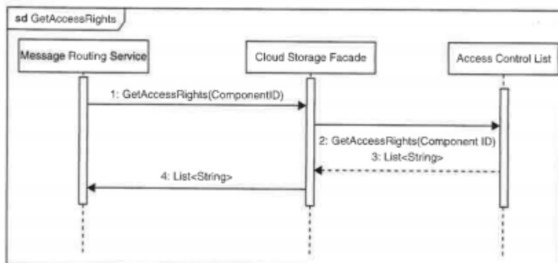
Figure 16.5 GetAccessRights
