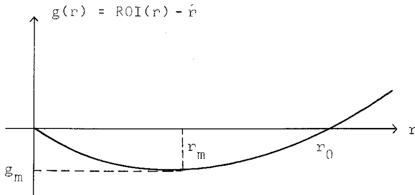
Figure 2.1. The difference g(r) as a function of the internal rate of return, r .
