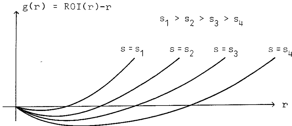
Figure 2.2. The effect of inflation on the difference function g(r) .
