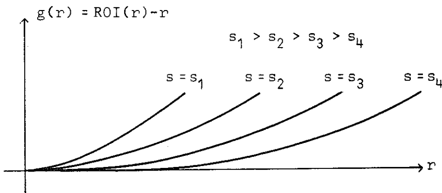
Figure 2.3. The effect of inflation on the difference function g(r) .
